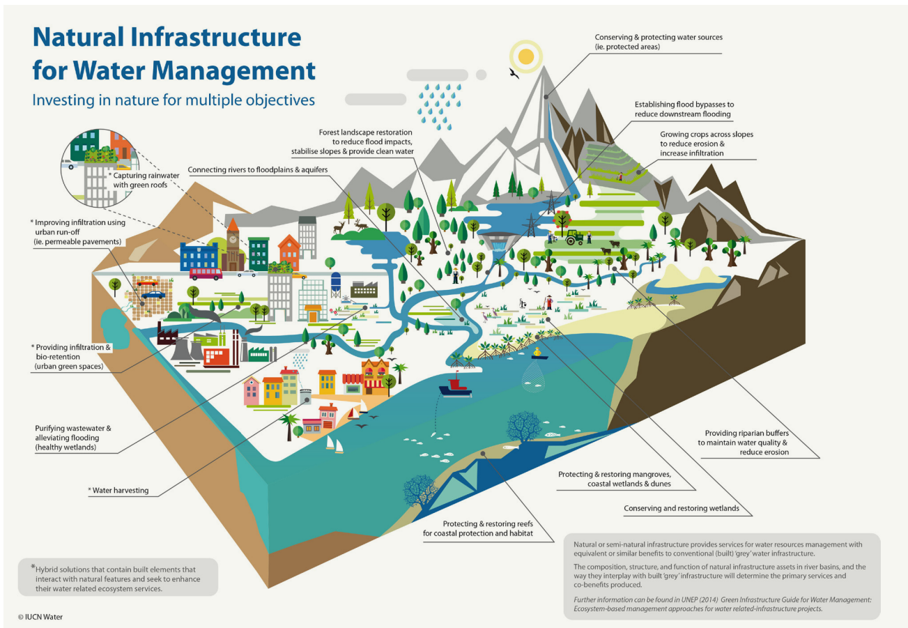
FIGURE 2. Diagram illustrating how green and grey infrastructure can work together—e.g., nature-based solutions (protection, revegetation) upstream, agricultural best management practices midstream, and grey infrastructure (treatment plant)/Sustainable Urban Drainage System downstream.
